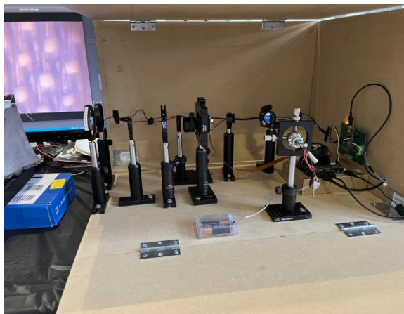
Figure 5: Overall Setup
